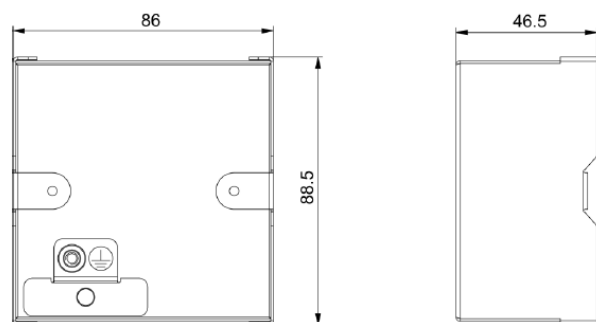
Fig.1.3 Dimension of Wiring Box Installed in Wall
