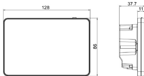
Fig.1.2 Dimension of Centralized Controller
